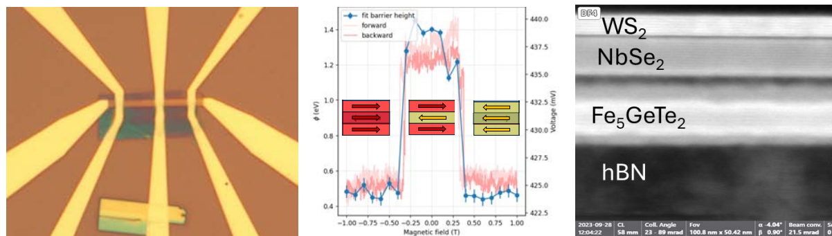
Figure (left) a Pt/few-layer CrSBr/Pt device made by Pierre-Eloi Paret, which showed tunnel barrier behaviour. (centre) Fine control of the CrSBr magnetisation with an applied magnetic field along the b axis. (right) TEM cross-section of a SC/M device made by Maya Klang, showing clean interfaces between the materials.
