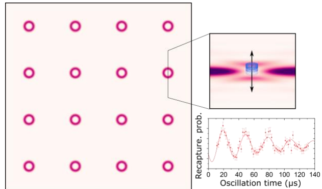
Individual circular Rydberg atoms are trapped in an array of optical bottle beams.
