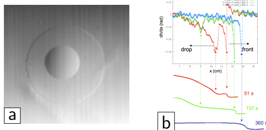
(a) Left-right slope of a drop of surfactant and its environment, showing a clearly marked circular swelling front. (b) The radial slope profile shows a wave that propagates without changing width or amplitude.
