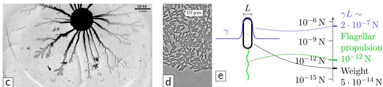
(c) Dendritic spreading of bacteria from a central inoculum by mass swarming. The gel surface is seen from above. (d) Tip of a dendrite at high magnification, showing the sharp boundary. (e) Capillary forces dominate by several orders of magnitude the propelling forces of the bacteria..
